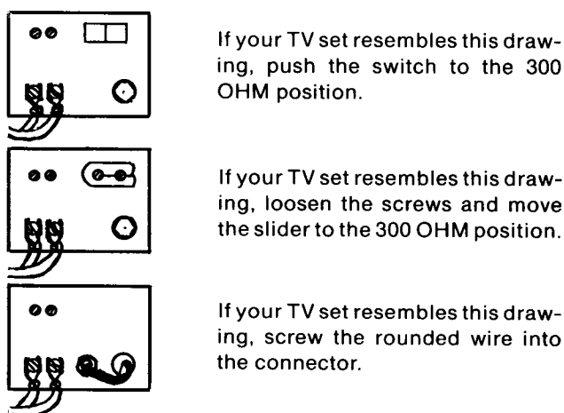
Figure 2.4. 300 OHM conversion
