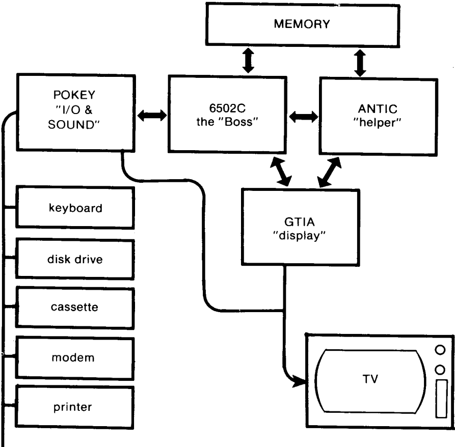
Figure 1.5. Inside the Atari
