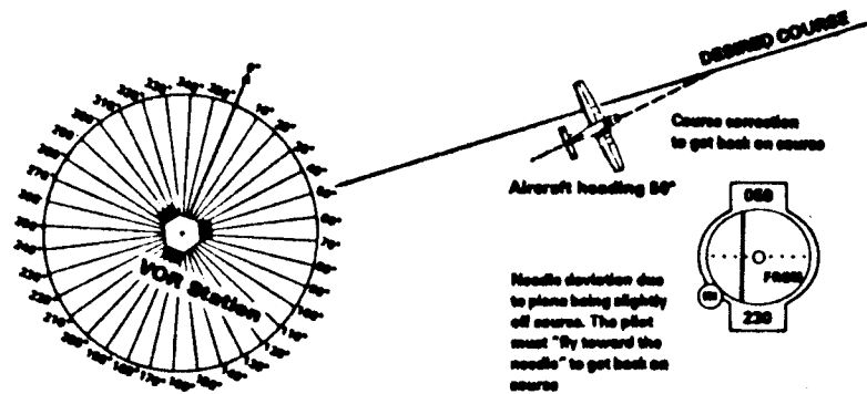
Figure 13. Flying from a VOR Station
