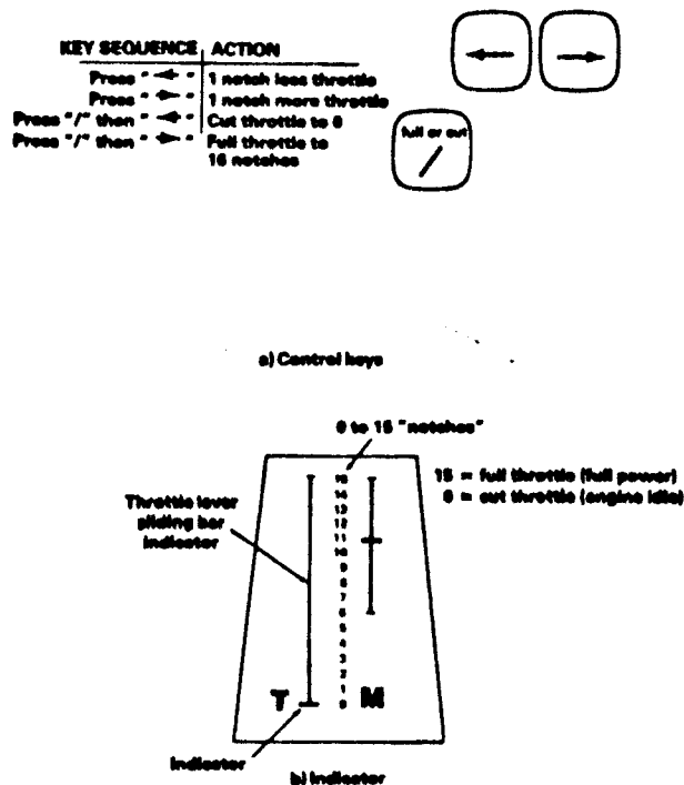
Figure 6. Throttle—Controls and Indicator
