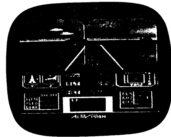
LANDING SCREEN
