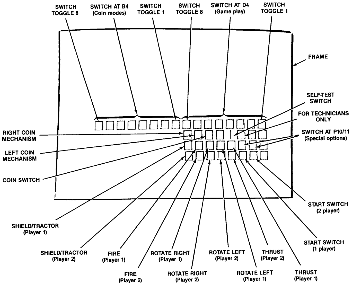
Figure 1-4 Self-Test Display
