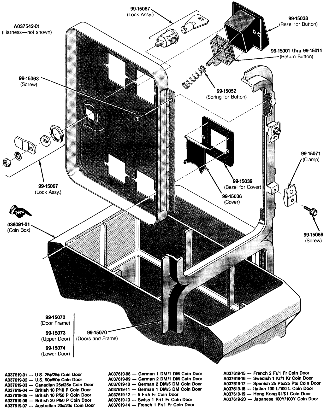
Figure 3-6 Vertically Mounted Coin Door, continued A037619-xx D
