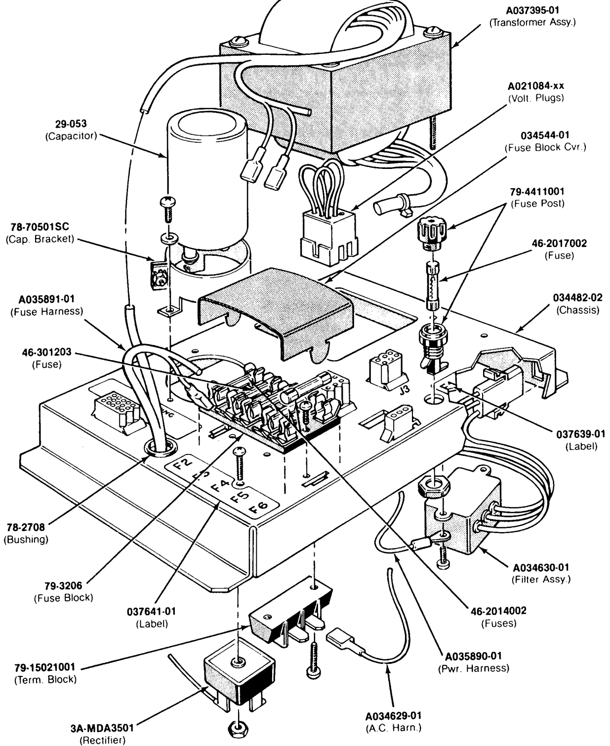
Figure 3-10 Color X-Y Power Supply Assemblies A037396-xx B
