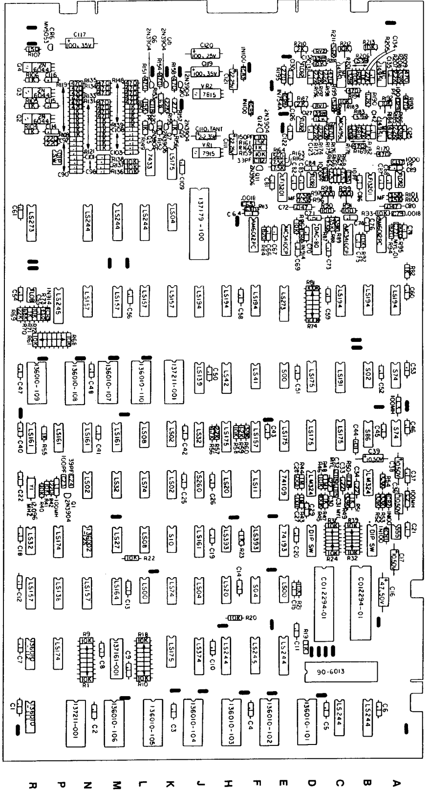
Figure 3-8 Gravitar™ Game PCB Assembly A038398-21 & -22 A
