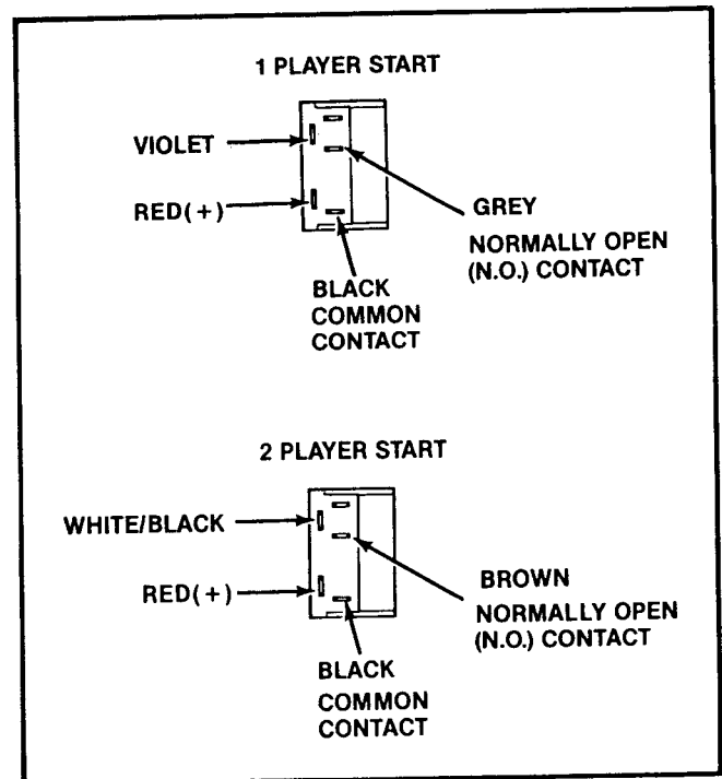
Figure 3-2 Control Panel
