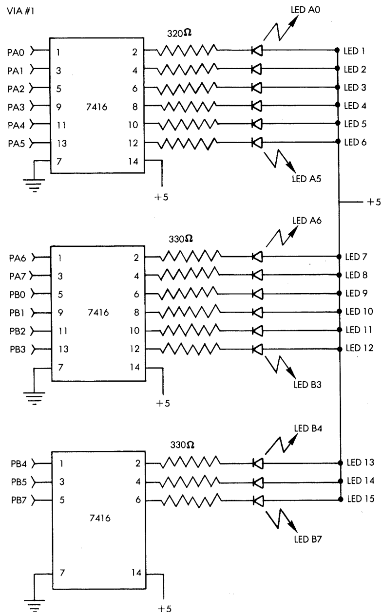
Fig. 3.5: LED Connections
