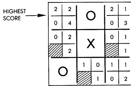
Fig. 11.25: Potential Evaluation
