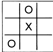
Fig. 11.18: Test Case 1
