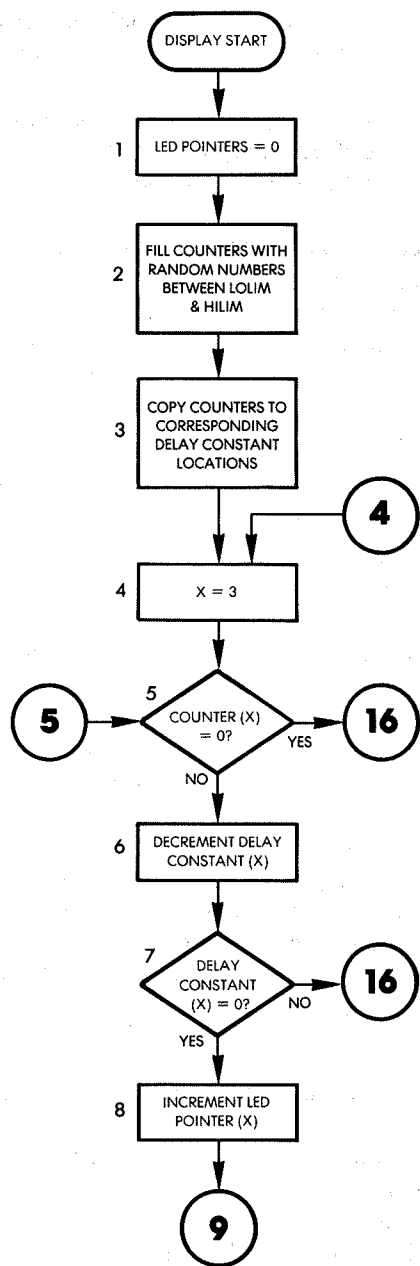
Fig. 7.4: DISPLAY Flowchart
