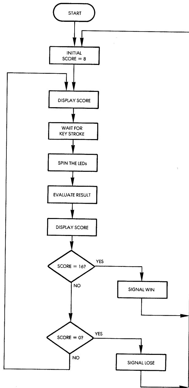
Fig. 7.3: Slots Flowchart
