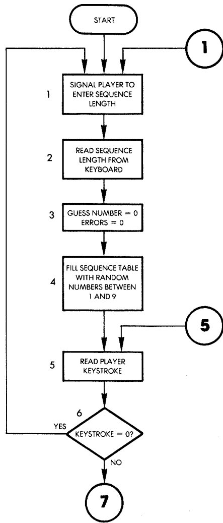
Fig. 8.4: Echo Flowchart
