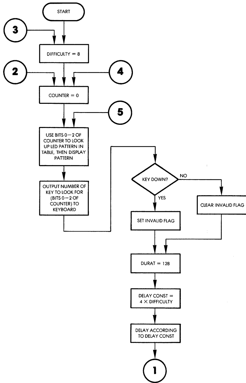
Fig. 6.1: Spinner Flowchart
