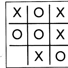
Fig. 11.11: Move 4
