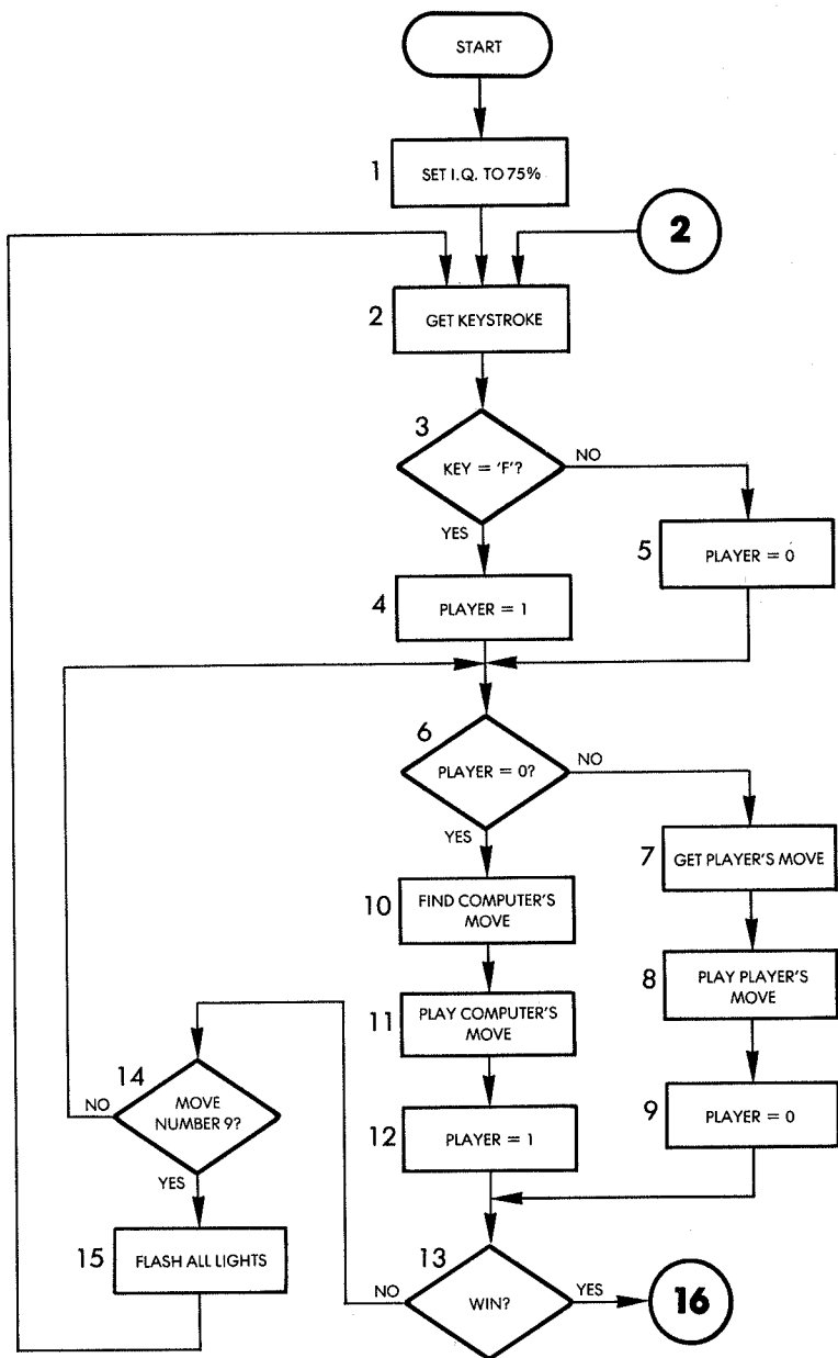
Fig. 11.45: Tic-Tac-Toe Flowchart
