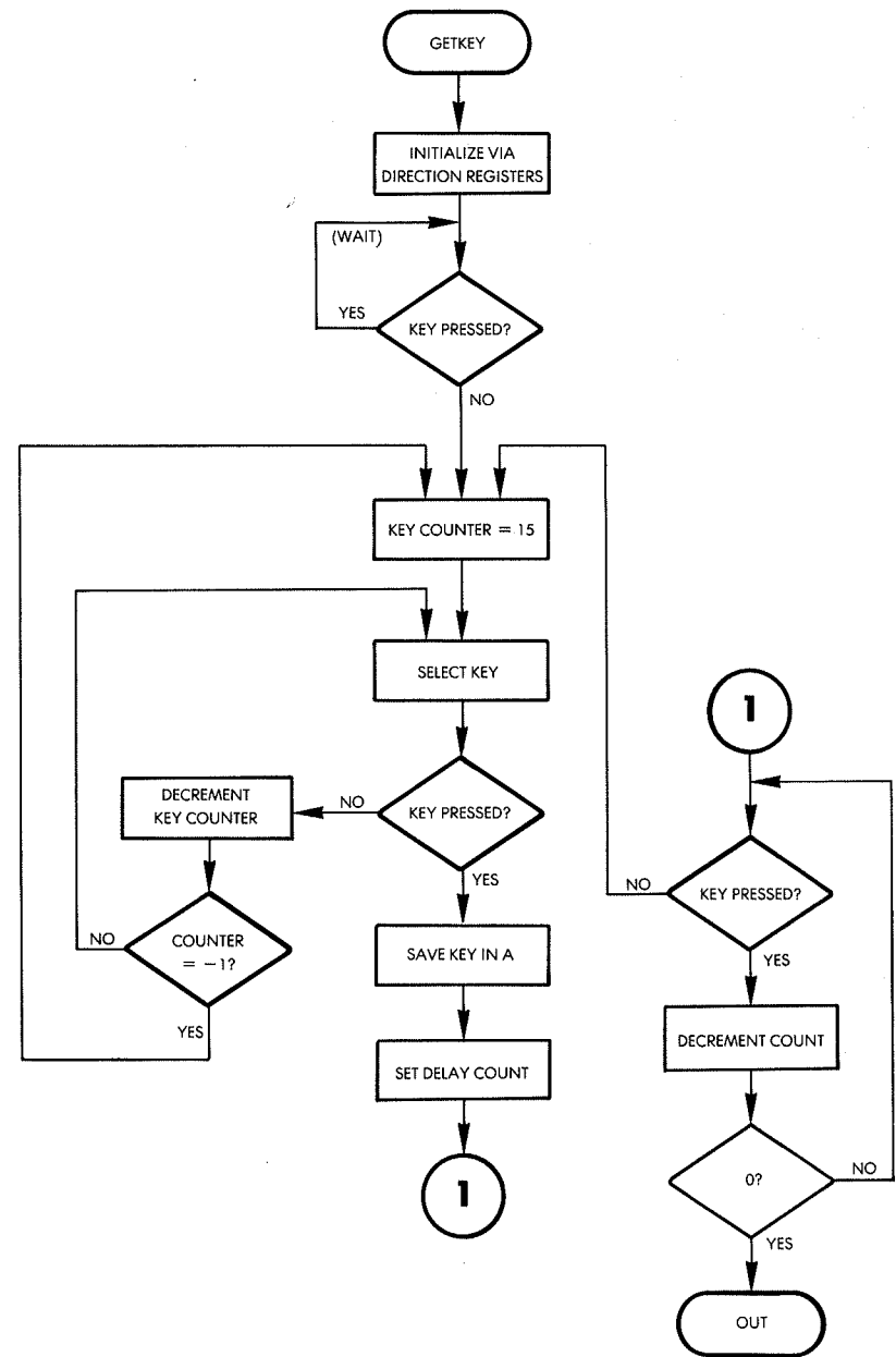
Fig. 1.16: GETKEY Flowchart
