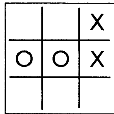
Fig. 11.9: Move 2
