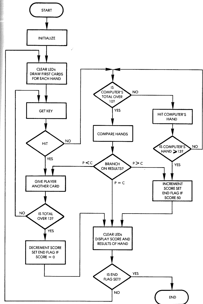
Fig. 10.9: Blackjack Flowchart
