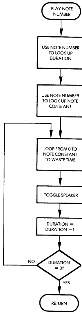
Fig. 2.8: PLAYIT Flowchart
