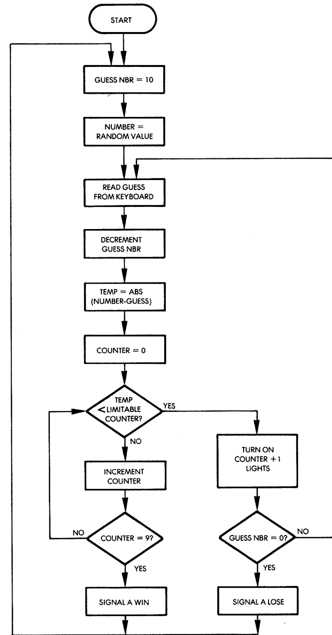
Fig. 4.1: Hexguess Flowchart
