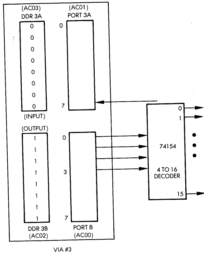
Fig. 1.15: VIA Connection to Keyboard Decoder
