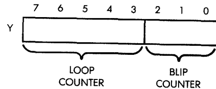
Fig. 6.2: Dual Counter
