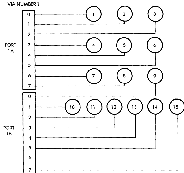
Fig. 1.13: Detail of LED Connection to the Ports
