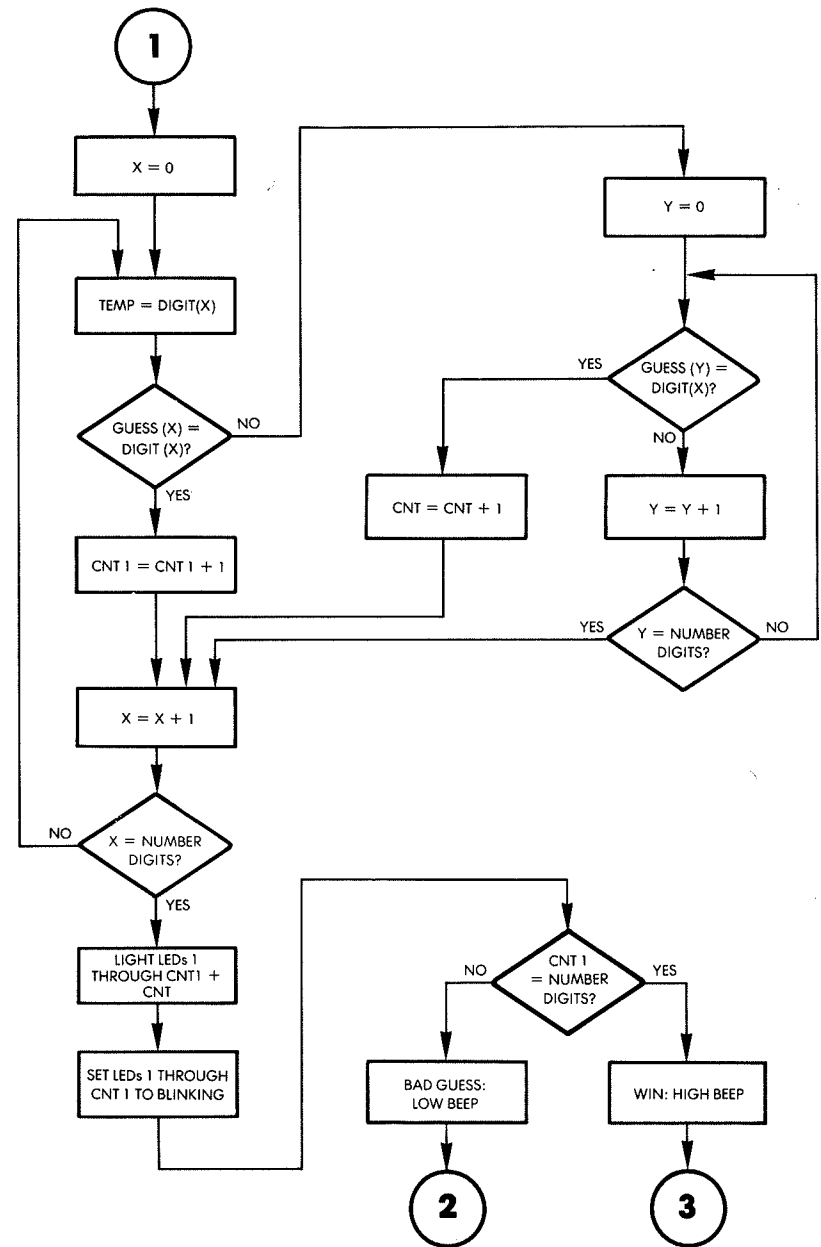
Fig. 9.9: Detailed Mindbender Flowchart (Continued)
