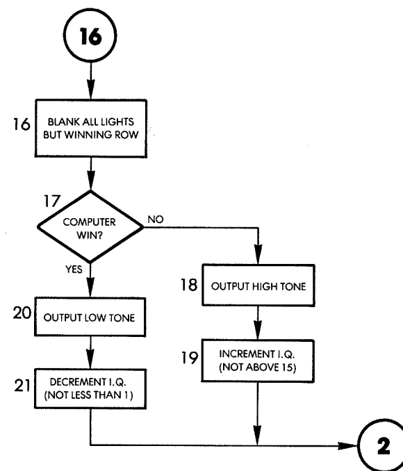
Fig. 11.45: Tic-Tac-Toe Flowchart (Continued)
