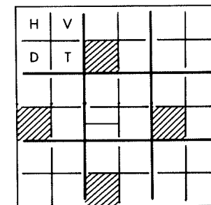
Fig. 11.17: Evaluation Grid
