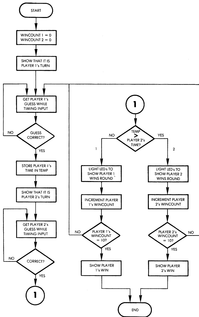
Fig. 3.4: Translate Flowchart
