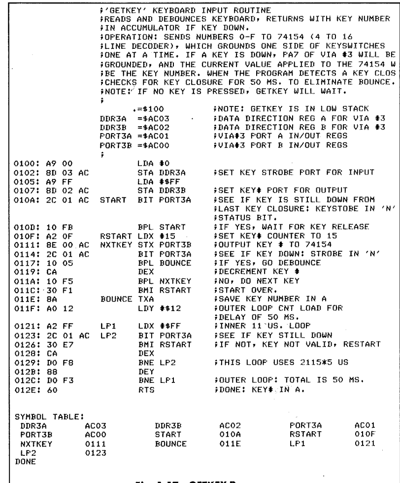
Fig. 1.17: GETKEY Program
