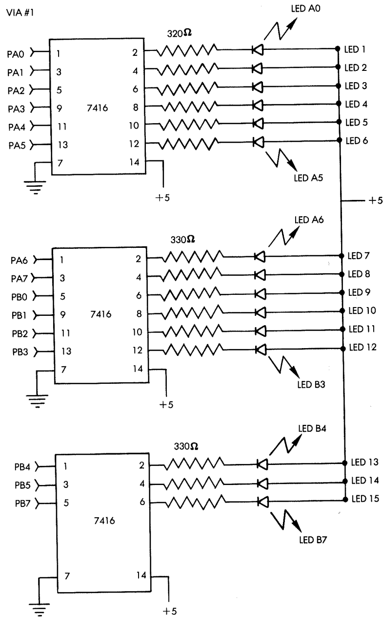
Fig. 1.11: LED Connection
