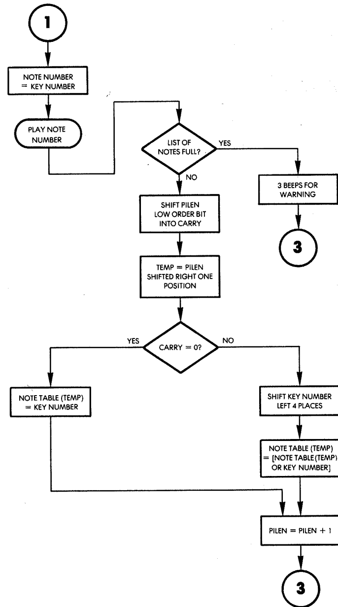
Fig. 2.7: Music Flowchart (Continued)
